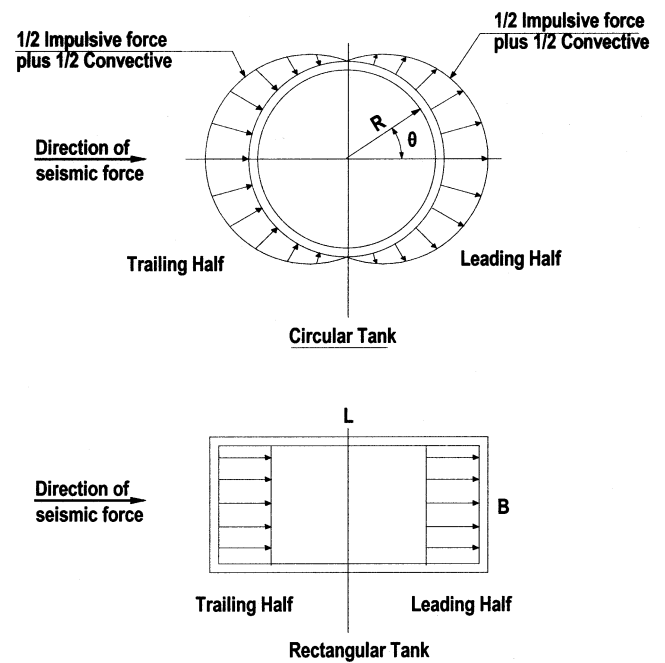
Fig. R5.2—Hydrodynamic pressure distribution in tank walls (adapted from References 3 and 13).
