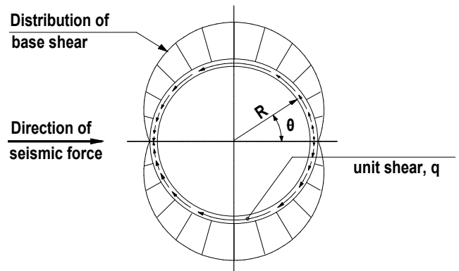
Fig. R5.1—Membrane shear transfer at the base of circular tanks (adapted from Reference 13).
