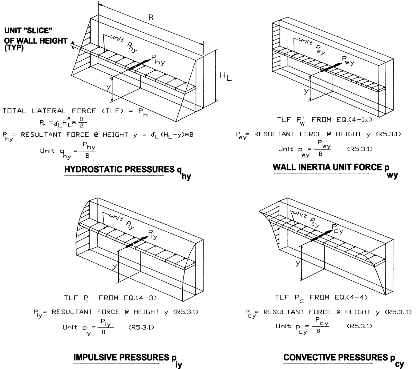
Fig. R5.4—Distribution of hydrostatic and hydrodynamic pressures and inertia forces on the wall of a rectangular liquid-containing structure (adapted from Reference 14).
