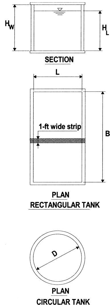
Fig. R2.1—Typical tank configurations (adapted from Reference 4).
