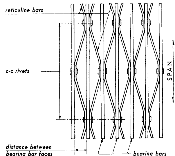
RIVETED GRATING
